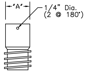
Overhead Connector (1)
