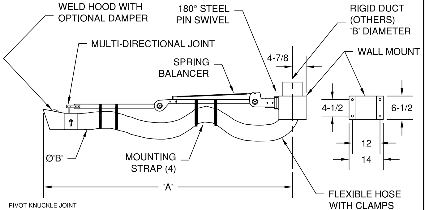
PIVOT KNUCKLE JOINT
