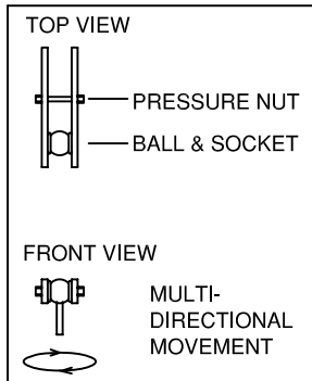
PIVOT KNUCKLE JOINT
