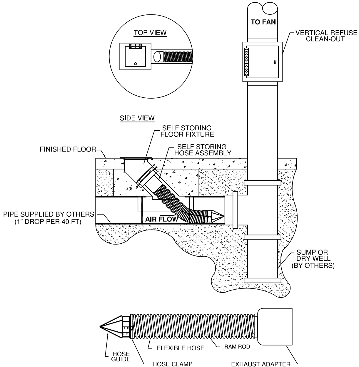
UNDERFLOOR SELF STORING HOSE ASSEMBLY
